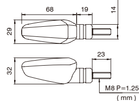
TYPE-602 LED FLASHER
