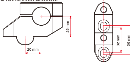
Bar rise kit offset dimension
