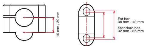
Bar rise kit dimension
