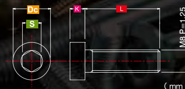
Caliper Bridge Bolt (mm)
