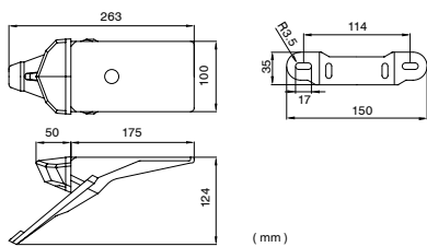
EDGE-2 TAIL LIGHT HOLDER Plastic Universal type
