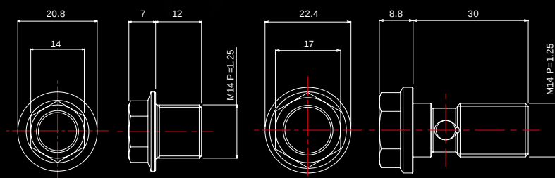
SUZUKI Engine Plug
